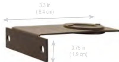
GUTTERMOUNT Aged Brass Gutter Mount
