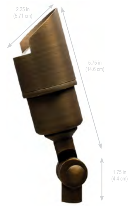
BL110-LED6W (6 watt MR16 LED lamp included)
