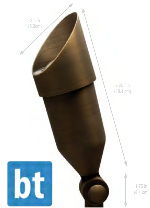
BL200-LED6W (6 watt MR16 LED Lamp included)
